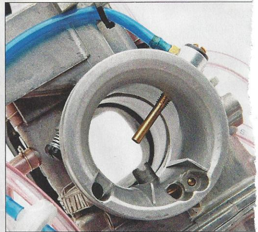
Dick's Racing can supercharge any two-stroke carb with its dual-fuel mod.
