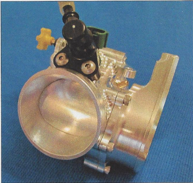
R&D Racing is working on a prototype throttle body that replaces the butterfly with a better flowing cam design.
